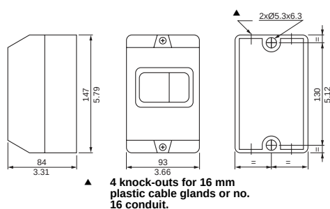
Surface mounting enclosure GV2MC0*
