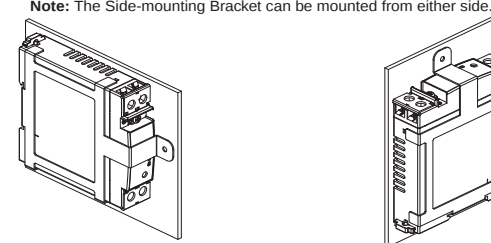
Horizontal mounting with S82Y-VS30P*
