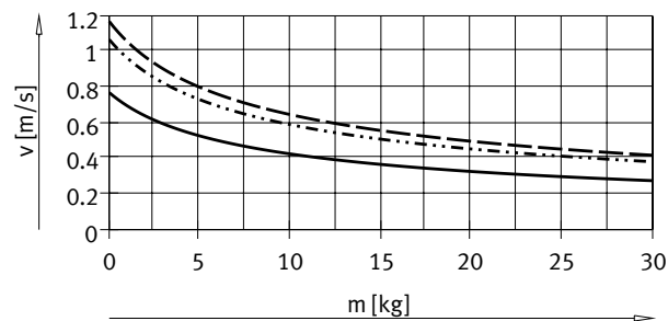
Average piston speed v as a function of payload m in combination with cushioning PPS
