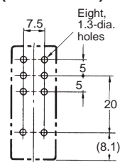
Mounting Holes (Bottom View)
