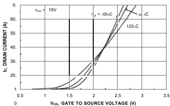
Figure 5. Transfer Characteristics.
