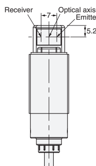
Suitable models E3RB-R□11 E3RB-D□1□
