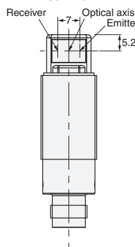
Suitable models E3RB-R□21 E3RB-D□2□
