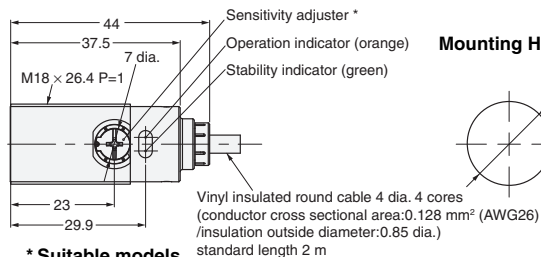
* Suitable models E3FB-T□11-D E3FB-R□12 E3FB-D□1□
