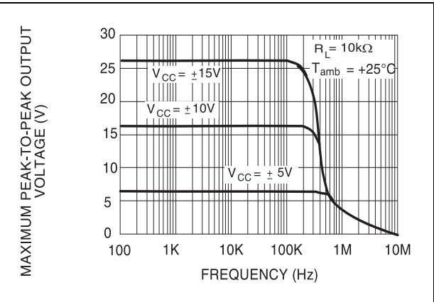
Figure 3. Maximum peak-to-peak output voltage versus frequency ( R_L = 10\text{ k}\Omega )
