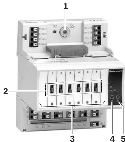
Fig. 19. XFR824 Panel Bus Relay Output Module (shown with terminal socket)
