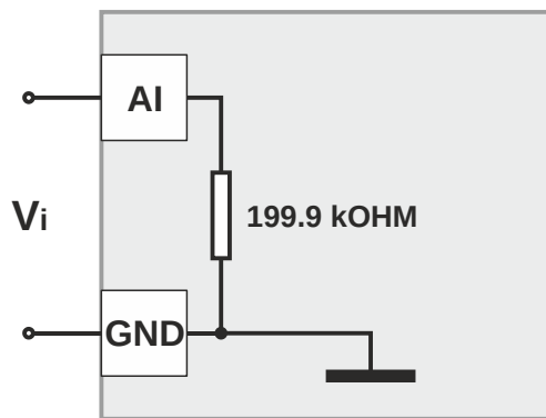
Fig. 30. Analog input high impedance (input circuit for voltage input for active sensors)
