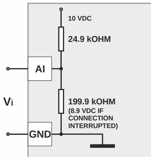
Fig. 31. Analog input impedance setpoint (input circuit for NTC10k \Omega , NTC20k \Omega , wall module setpoint)
