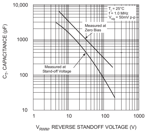
Fig. 3 Typical Total Capacitance
