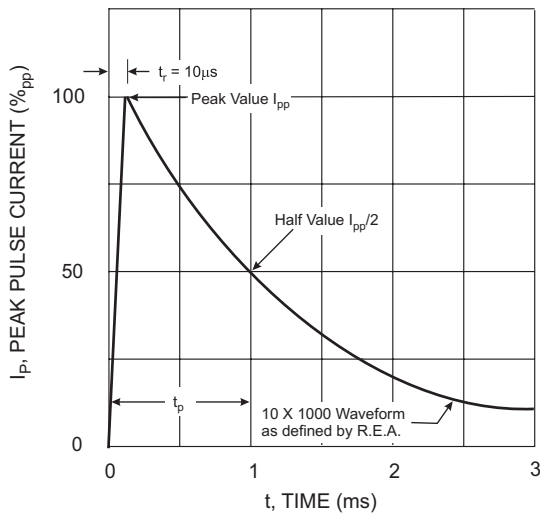
Fig. 1 Pulse Waveform
