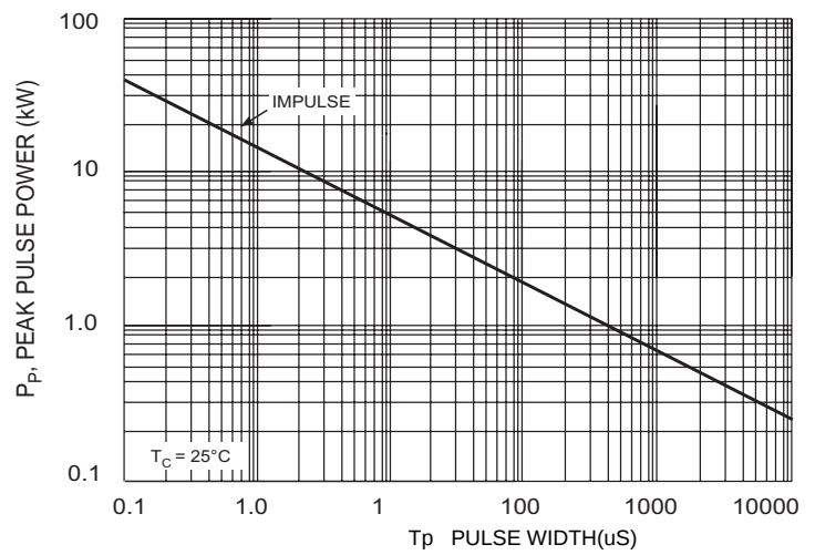
Fig. 2 Pulse Rating Curve
