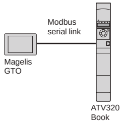
Example of configuration on Modbus serial link
