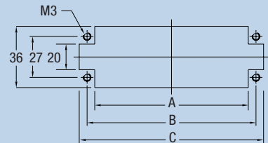
Panel cut-out
