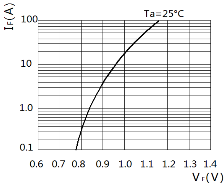
FIG.4-TYPICAL FORWARD CHARACTERISTICS
