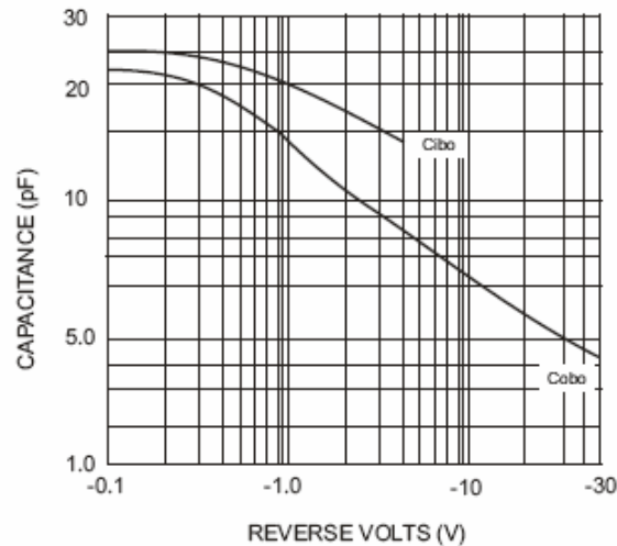
Fig. 1 Typical Capacitance
