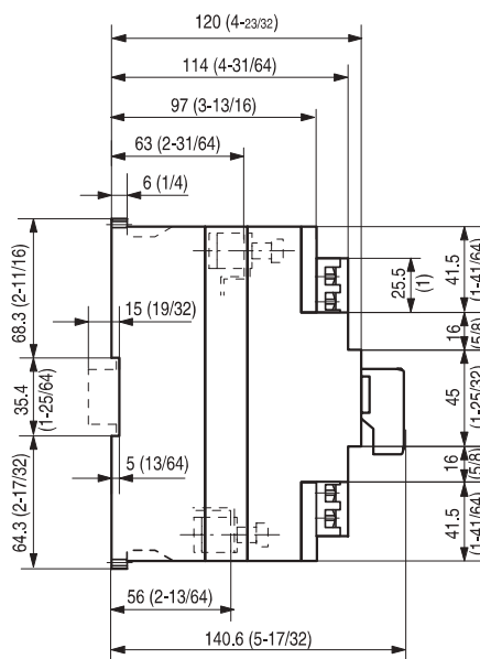
Mounting position 140-MN (KTA 3-25)
