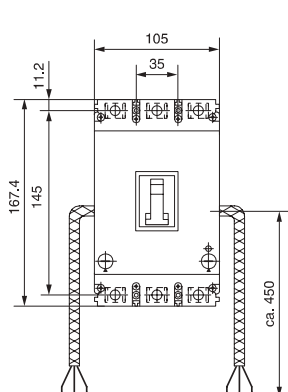
140M-K5F (KTA 3-160S)
