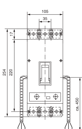
140M-M5F (KTA 3-250S)
