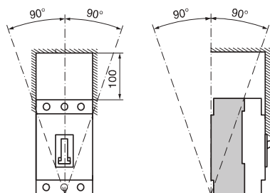
Mounting position / Safety Clearance 140M-K5F... 140M-P5F (KTA 3-160S... KTA 3-400S)
