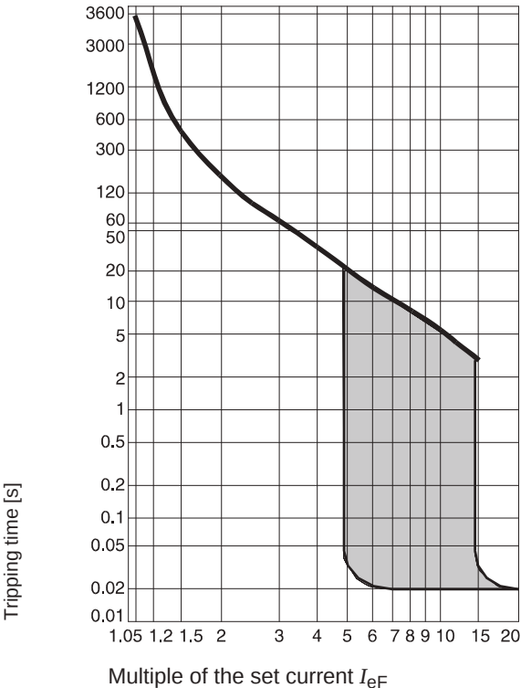
140M-M5F(4) (KTA 3-250S(4))
