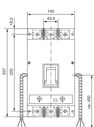
140M-P5F (KTA 3-400S)
