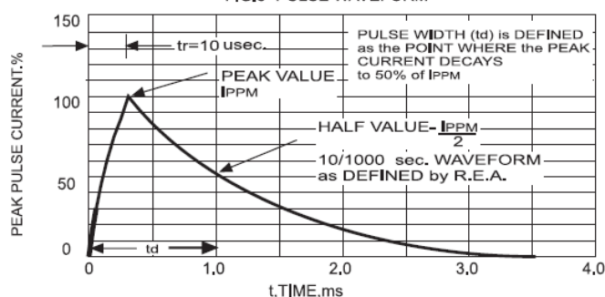
FIG.3- PULSE WAVEFORM
