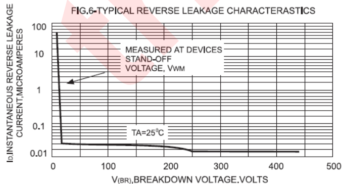
FIG.6-TYPICAL REVERSE LEAKAGE CHARACTERISTICS
