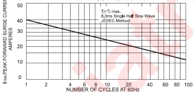
FIG.5-MAXIMUM NON-REPETITIVE FORWARD SURGE CURRENT UNIDIRECTIONAL ONLY
