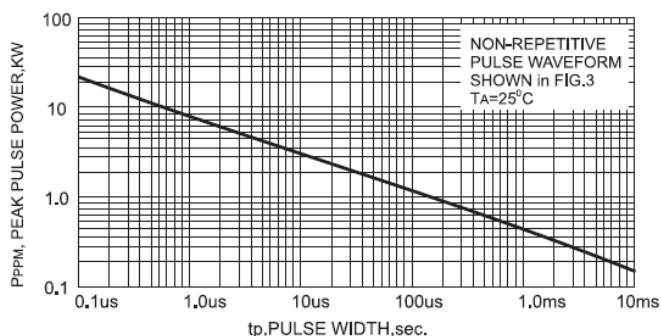
FIG.1- PEAK PULSE POWER RATING CURVE
