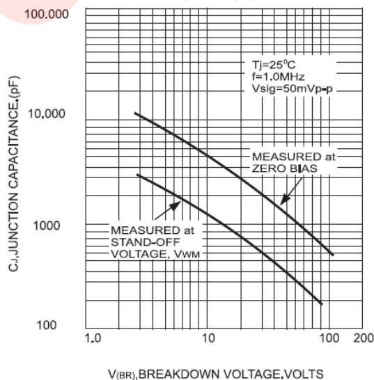
FIG.7-TYPICAL JUNCTION CAPACITANCE UNIDIRECTIONAL
