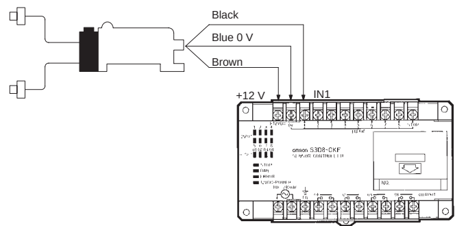
Connection with S3D8 Sensor Controller
