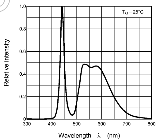
Fig. 8.6 Wavelength Characteristic
