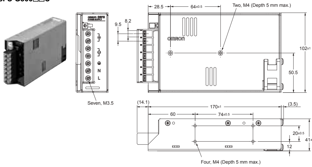
Panel mounting holes dimensions
