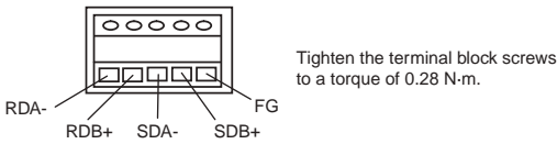
●RS-422A/485 Terminal Block
