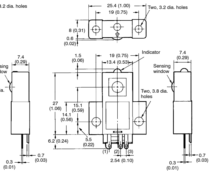
Receiver (EE-SPWD_11)
