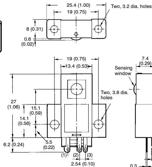
Emitter (EE-SPWL_11)
