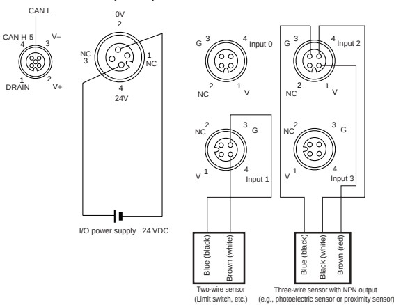
DRT2-ID04CL (NPN)
