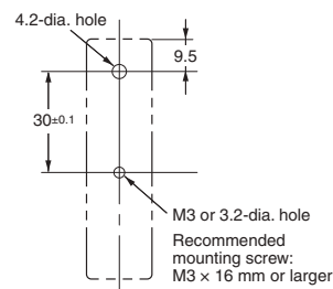
Mounting Hole Dimensions
