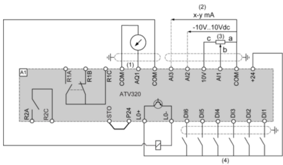
Control Connection Diagram in Source Mode
