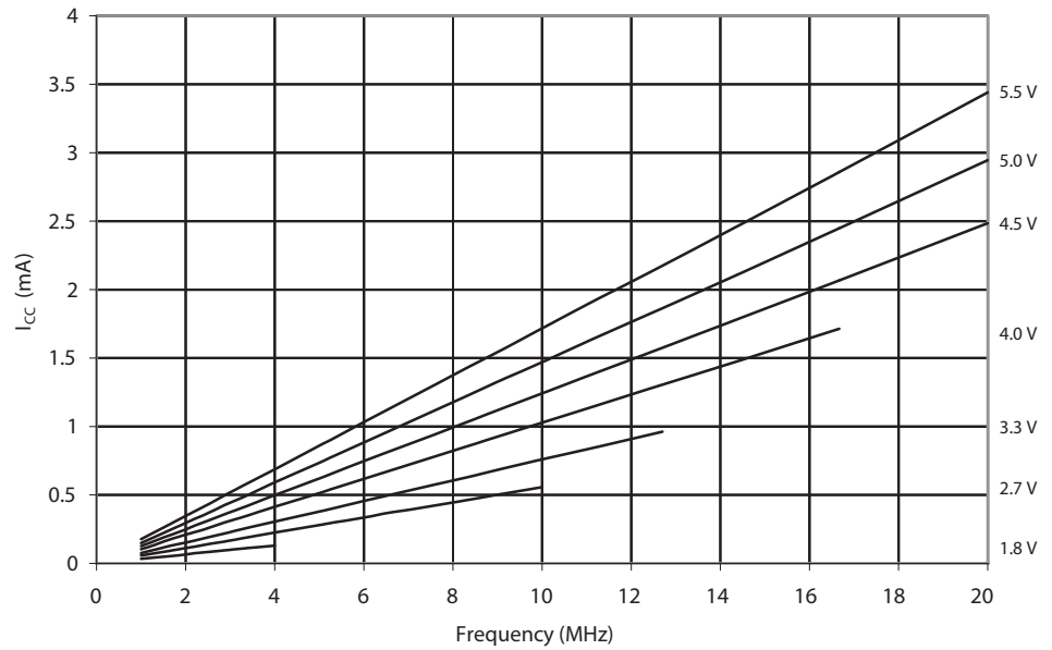
Figure 21-63. Idle Supply Current vs. V_{CC}
