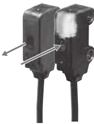
Emitter: E3T-STM-L Receiver: E3T-STM-D
