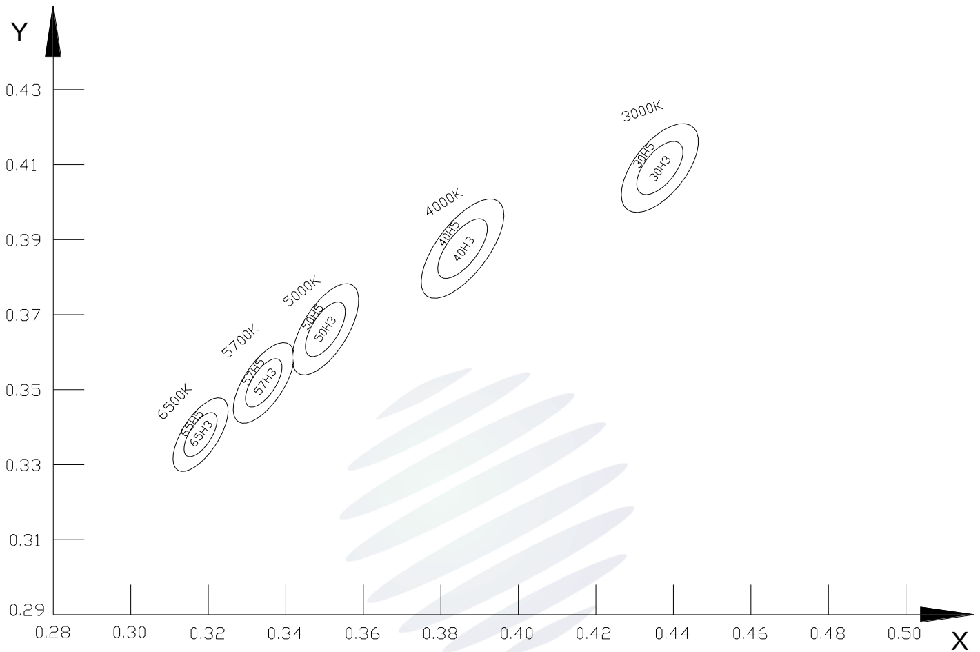
Fig 1-6 The C.I.E Chromaticity Diagram CIE色度图
