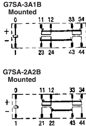
Terminal Arrangement/Internal Connection Diagram (Bottom View)
