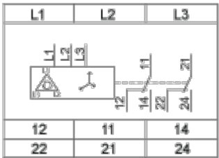
Wiring Diagram
