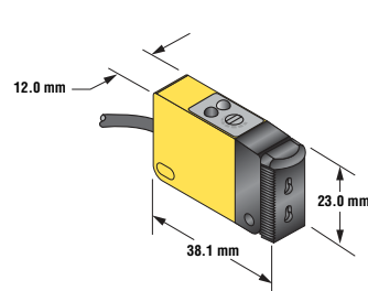
QH23 Plastic Fiber Optic Models Suffix FP and FPY
