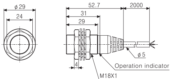
●PRDL18-7D□
