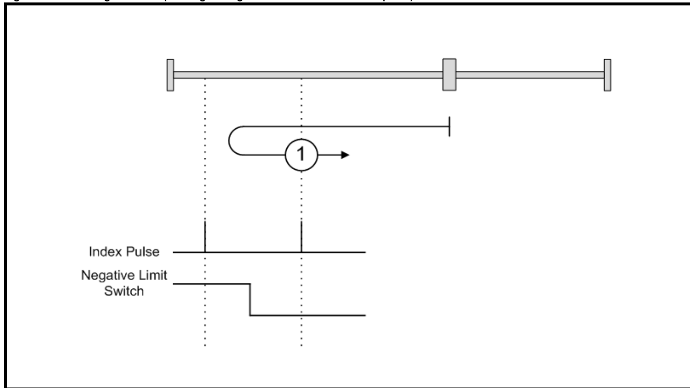
Figure 11-15 Homing method 1 (Homing on negative limit switch and index pulse)
