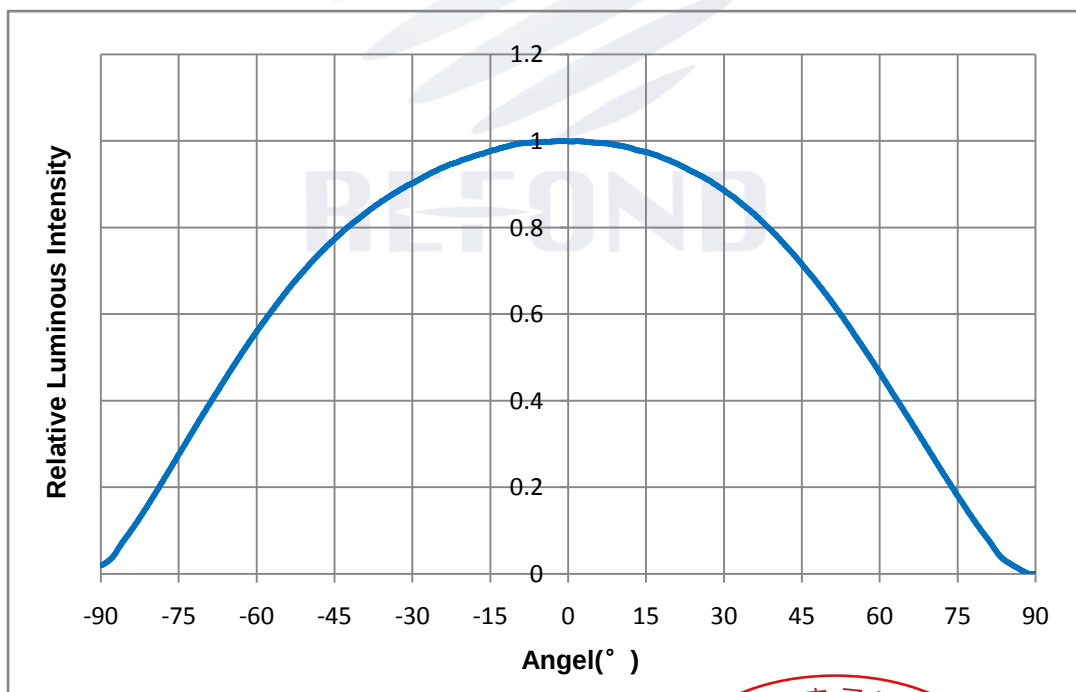
Fig 1-12 Radiation diagram
