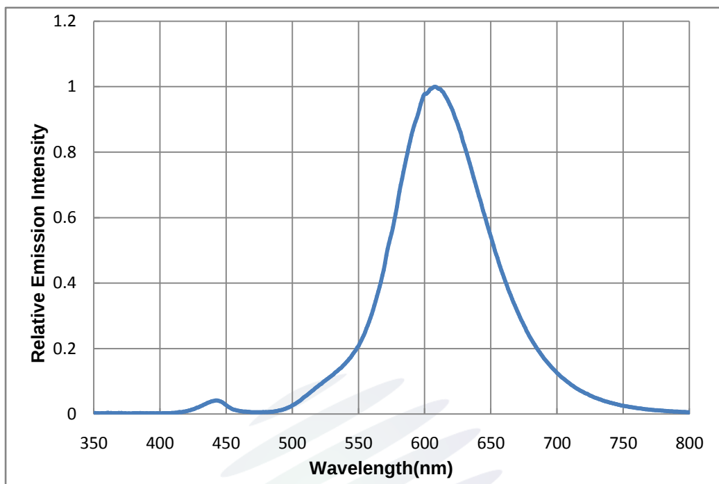
Fig 1-13 Spectrum Distribution
