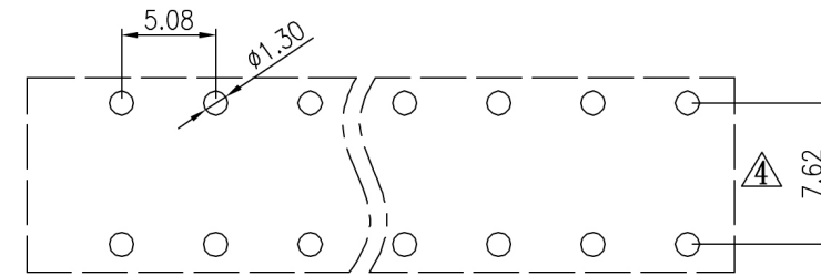
TOP VIEW-LAYOUT
